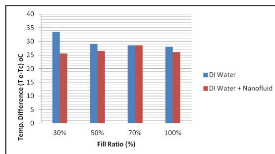
Fig.4. Temperature vs. fill ratio for different working fluids for input heat of 8W
