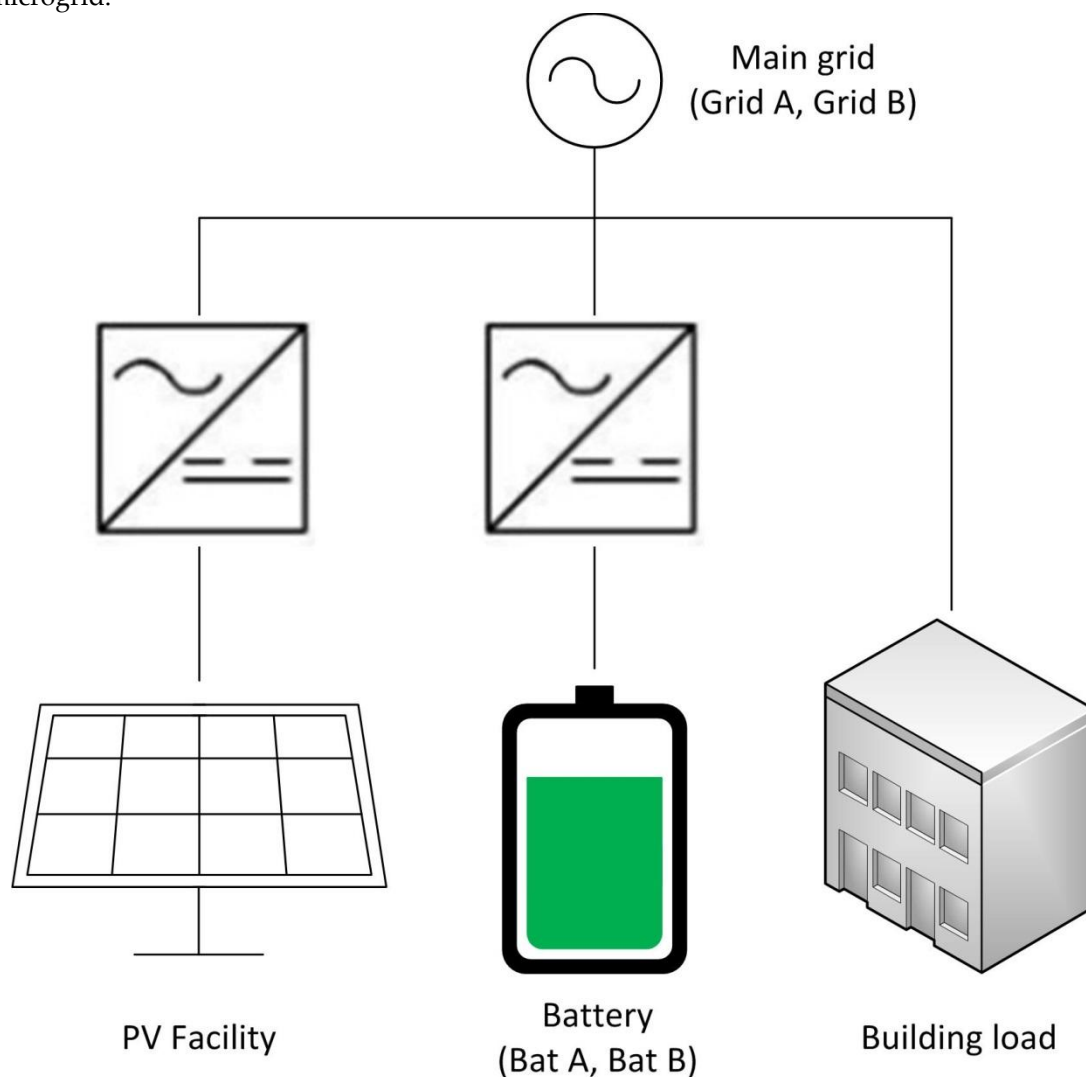
Figure 1. Microgrid model.
