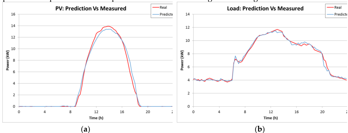
Figure 9. Predictions and actual values for (a) the PV generation and (b) the loads.
