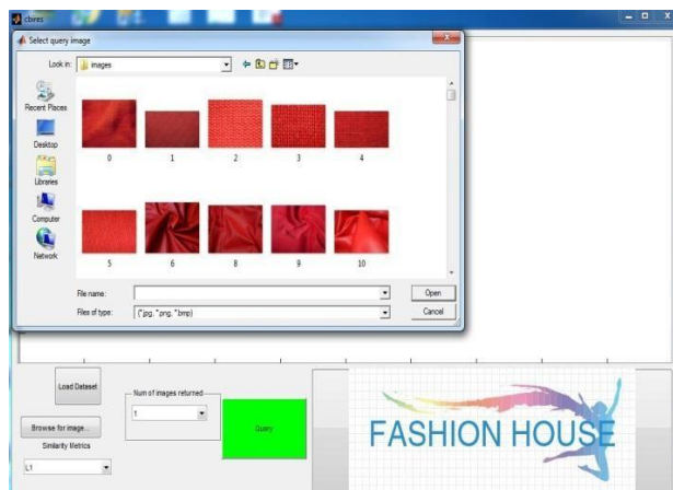
Figure 3.load query image
