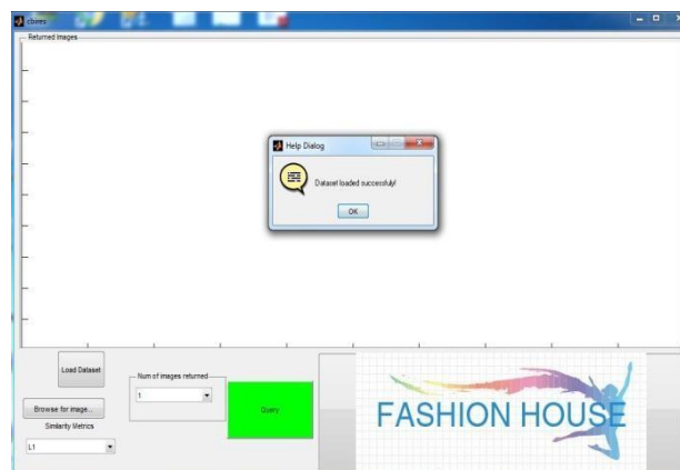
Figure 2. load dataset
