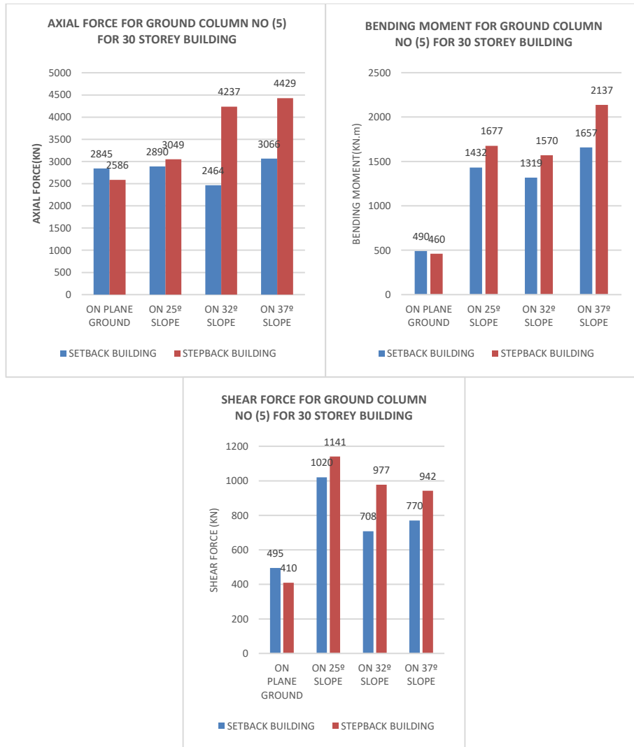
❖ 30 storey set back and step back building forces comperission for ground column no six(6)
