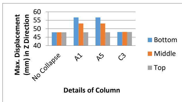
Fig. 4.4: Maximum Displacement (mm) in Z direction at various stories
