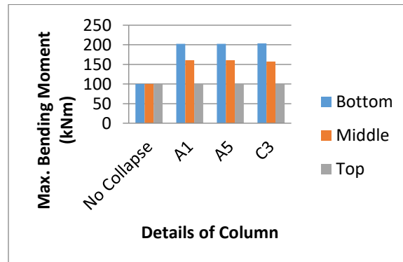
Fig. 4.1: Maximum bending moment M_z (kNm) at various stories
