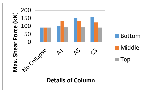
Fig. 4.2: Maximum Shear Force (kN) at various stories
