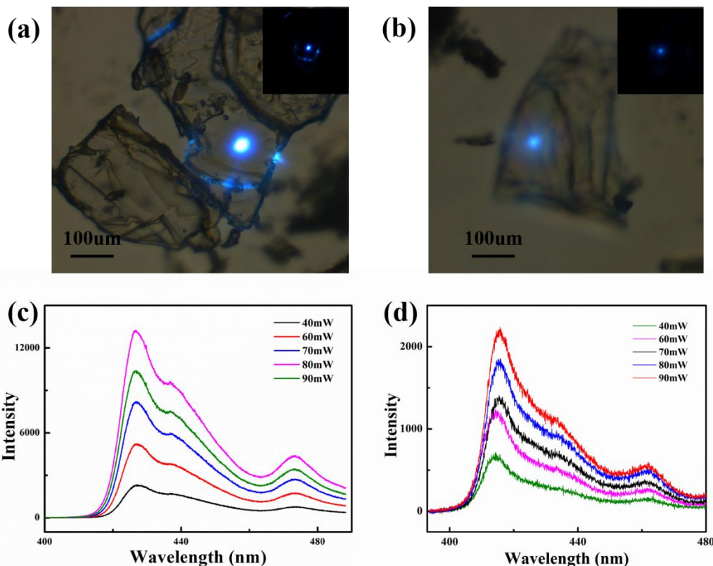
Figure 6. The optical microscope images of the perovskite (a) (C_4H_9NH_3)_2PbBr_4 ; (b) (C_6H_5CH_2NH_3)_2PbBr_4 ; the two-photon PL spectrum of the perovskite (c) (C_4H_9NH_3)_2PbBr_4 ; (d) (C_6H_5CH_2NH_3)_2PbBr_4 .
