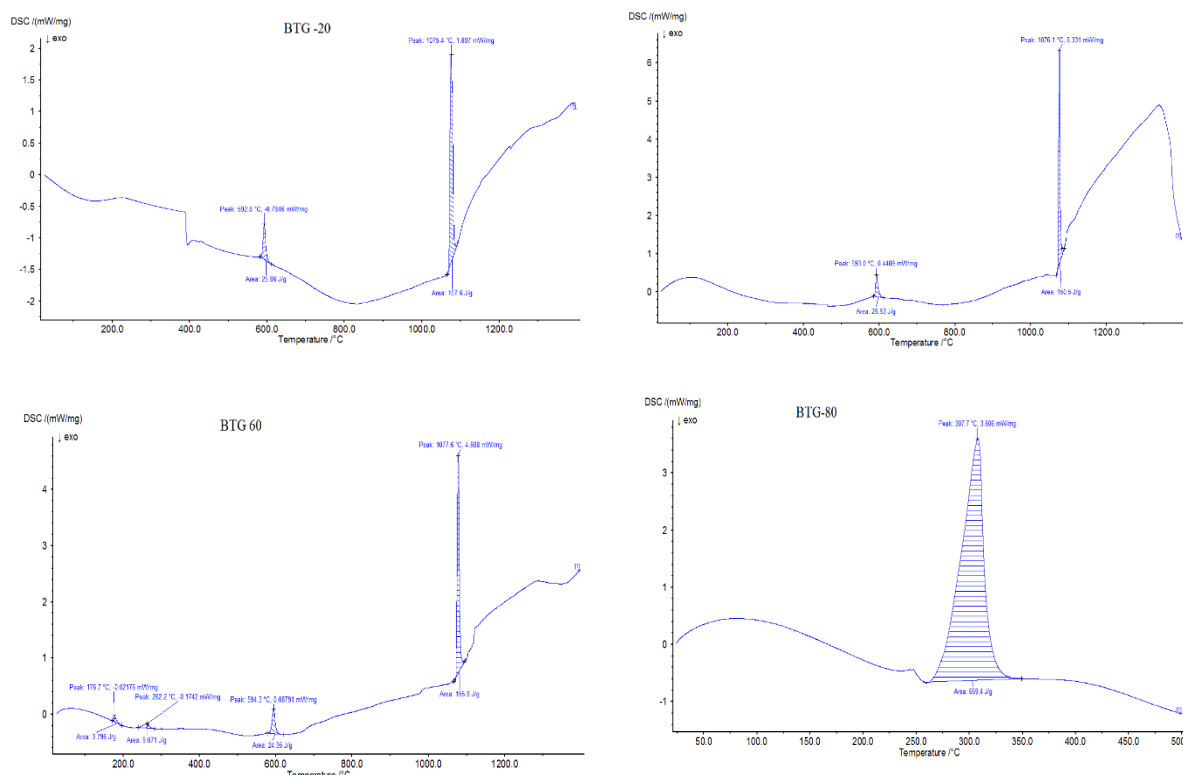
Fig 7 - Differential Thermal Analysis curves of LAPS crystals
