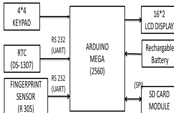
Fig.4. Block Diagram
