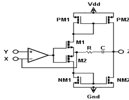
Fig. 2. CCII+ block with series-RC compensation.
