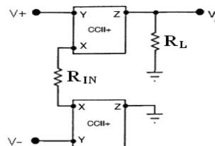
Fig. 5. 2-CC schematic design [3].
