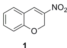
Figure 1. Structure of 3-nitro-2H-chromene 1
